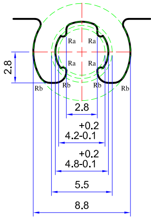
Detail 'K9' Scale 3:1
